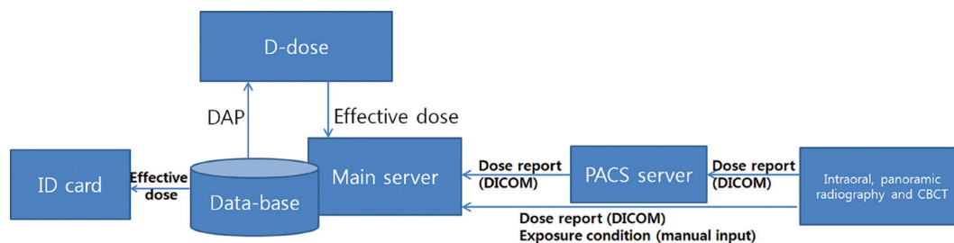
Fig. 3. Schematic view of the dose report transfer, conversion, and store process in the dose monitoring system.
