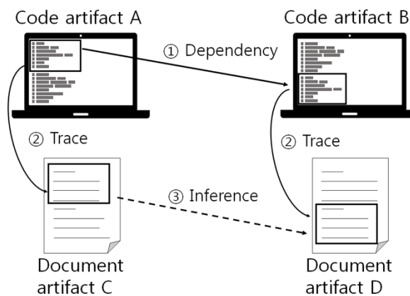
Fig. 3. A traceability link graph between code artifacts and document artifacts
