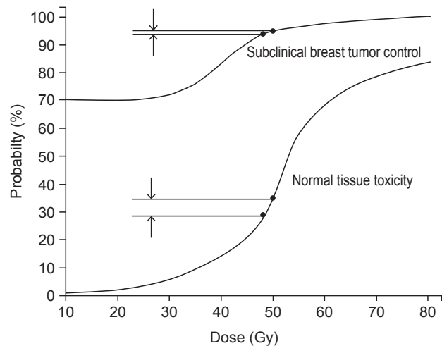
Fig. 1. Dose-response curve for subclinical breast tumor control and normal tissue toxicity. Yarnold et al. [22] mentioned that small decrease in total dose allows greater decrease in normal tissue toxicity under the acceptable compromise of local control considering different steepness of the two curves.
