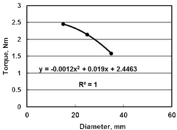
Fig. 11. Relationship between tube diameter and applied torque for CCT test.
