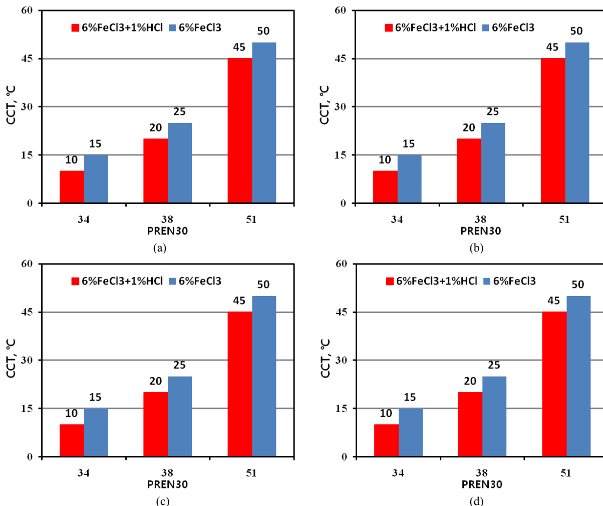
Fig. 9. CCT of the austenitic stainless steels determined in 6% FeCl 3 + 1% HCl and 6% FeCl 3 solution; (a) plate, and (b) round bar (D; 35 mm), (c) round bar (D; 25 mm), (d) round bar (D; 15 mm).
