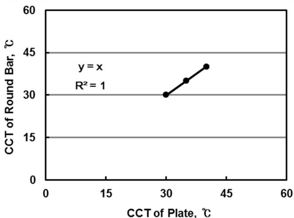
Fig. 8. Relationship between CCT of plate and CCT of cylindrical specimen (diameter; 25 mm).
