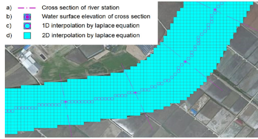
Fig. 1. Conceptual diagram of the process of distributing 2-dimensional water level from 1- dimensional water level. At the first, the cross section of river stations are determined, the position of center point is determined for the second, water surface elevation on the center line of river was interpolated by 1D Laplace equation for the third, and water surface elevation in the remaining area was interpolated by 2D Laplace equation for the last.
