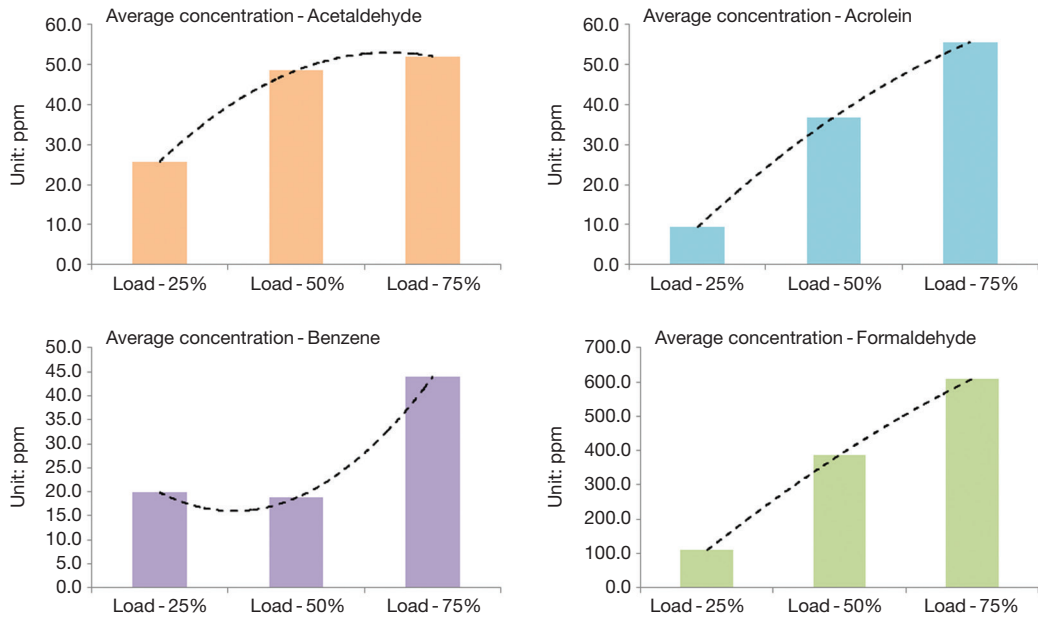
Fig. 4. Average concentration of VOCs by the engine load.
