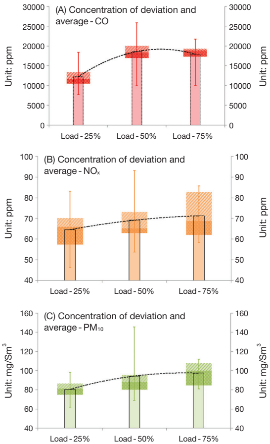
Fig. 3. Average concentration and deviation by the engine load.
