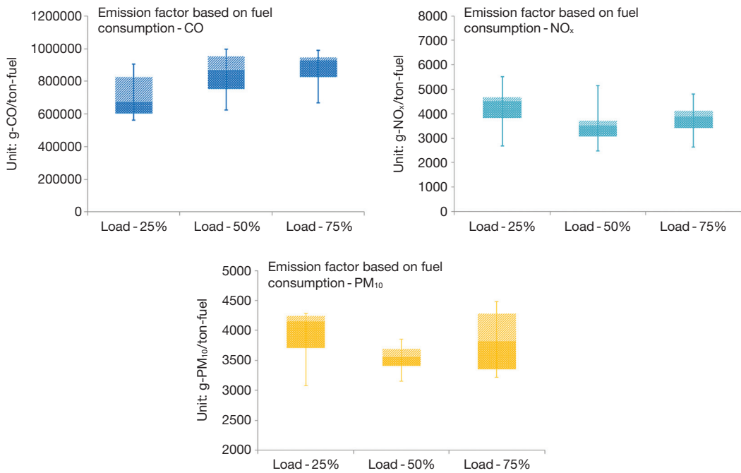
Fig. 5. Emission factor of pollutants based on fuel consumption.
