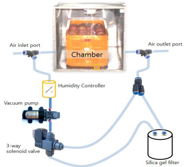
Fig. 2. Device used to control humidity in the chamber.
