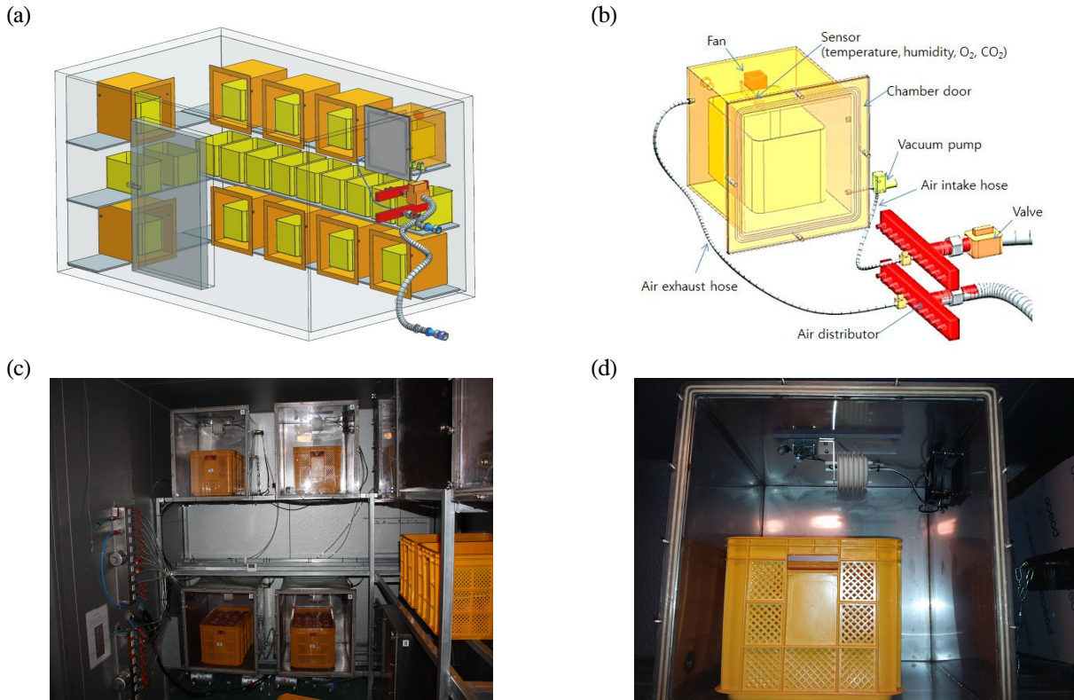
Fig. 1. Schematic views (a, b) and photos (c, d) of CA low temperature storage system (a, c) and gas control chamber (b, d).
