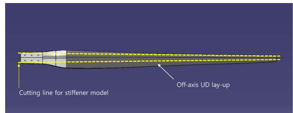
Fig. 7. Shape of blade stiffener scaled model
