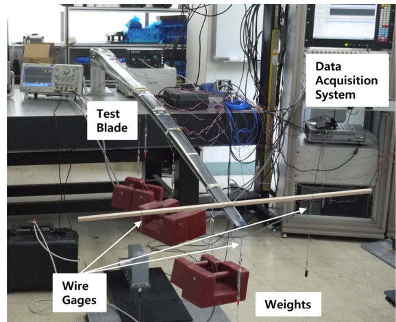
Fig. 8. Configuration of BTC static load experiment
