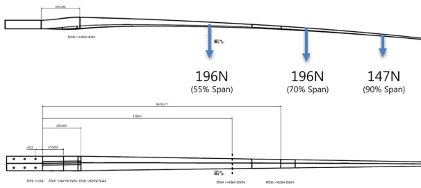
Fig. 9. Loading position of blade stiffener scaled model
