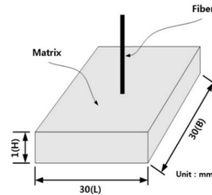
Fig. 3. Specimen geometry of fiber pullout test [12]
