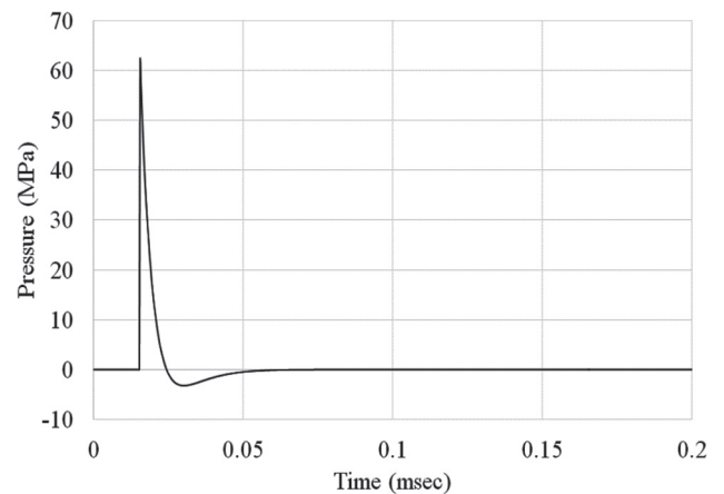
Fig. 2 Pressure diagram under 30 kg of TNT.
