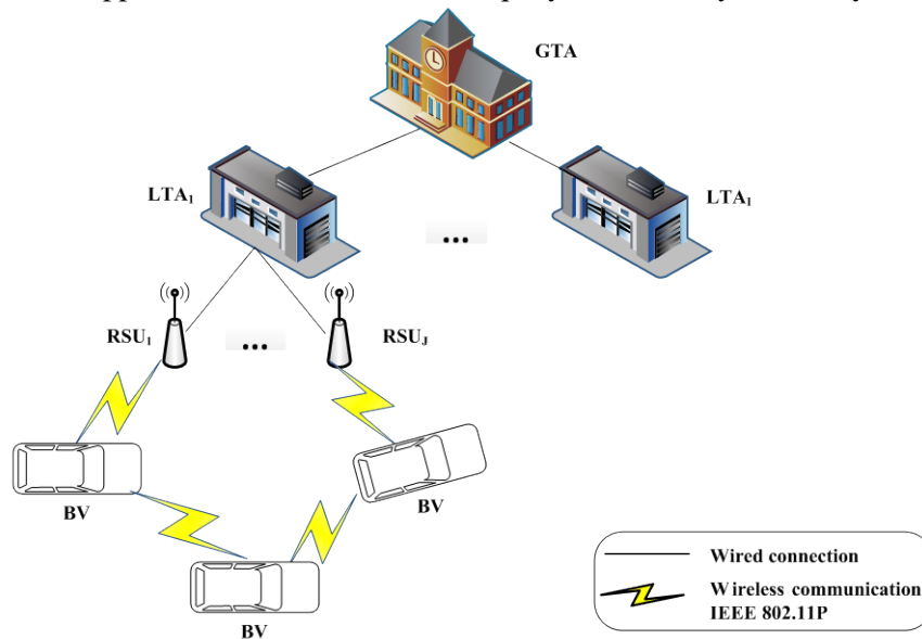
Fig. 1. System Model of VANETs
