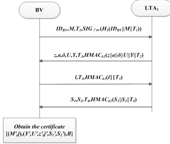
Fig. 2. Certificate Generation
