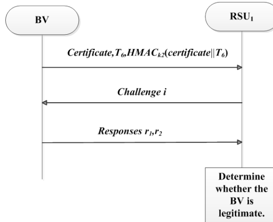
Fig. 3. Certificate Authentication
