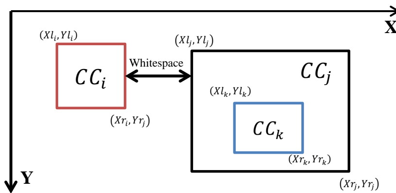
Fig. 2. Example of connected component analysis and whitespace extraction.
