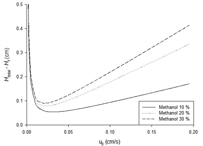
Fig. 5. Correlation between HETP and the flow rate upon changing the methanol ratio of the mobile phase.
