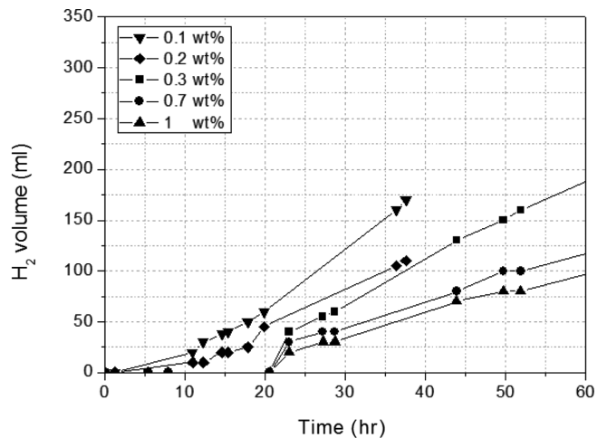
Fig. 1. Effect of NaOH concentration on the evolution rate of hydrogen during NaBH 4 storage.
