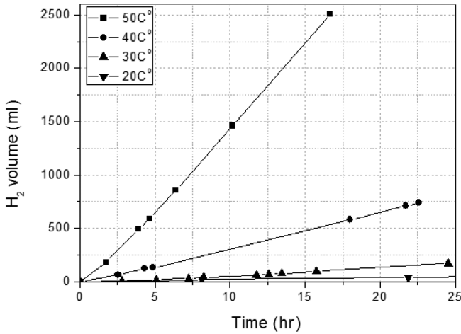
Fig. 2. Effect of temperature on the evolution rate of hydrogen during NaBH 4 storage with 0.3 wt% NaOH.
