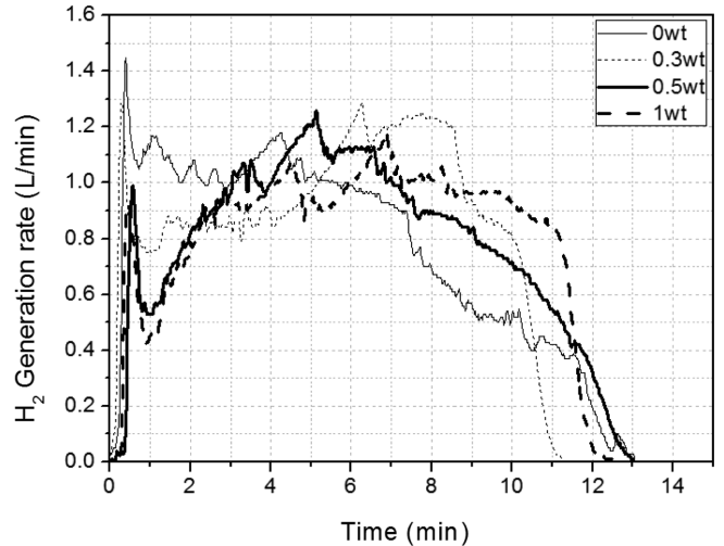
Fig. 7. Effect of NaOH concentration on the evolution rate of hydrogen during NaBH 4 hydrolysis reaction with Co-P-B catalyst at 80 °C.
