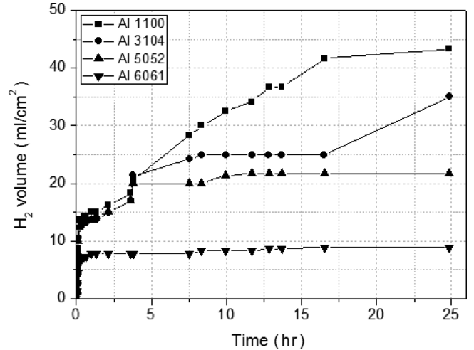
Fig. 4. Comparison of corrosion rate of aluminum alloys with 1.0 wt% NaOH at 80 °C.
