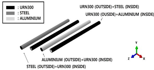
Fig. 2. Four types of hybrid pantographs for the parametric study
