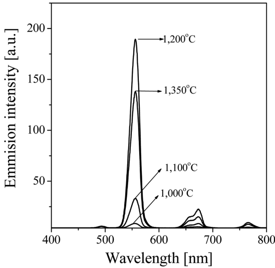
Fig. 3. Emission spectra (Sr 0.999 , Ho 0.001 )Al 2 O 4 UCP powders calcined at various temperatures.
