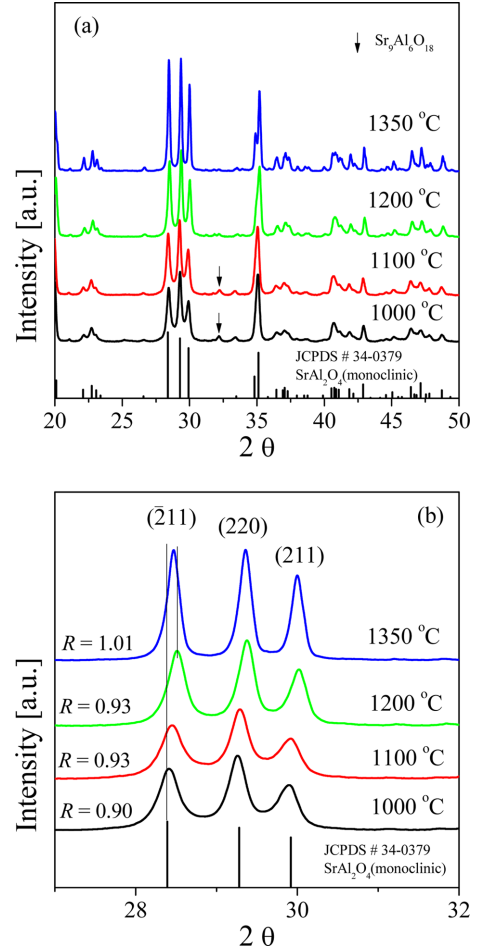
Fig. 2. XRD patterns of SrAl 2 O 4 :Ho 3+ UCP powders calcined at various temperatures: (a) full spectra (b) enlarged patterns for (-211), (220) and (211) planes.
