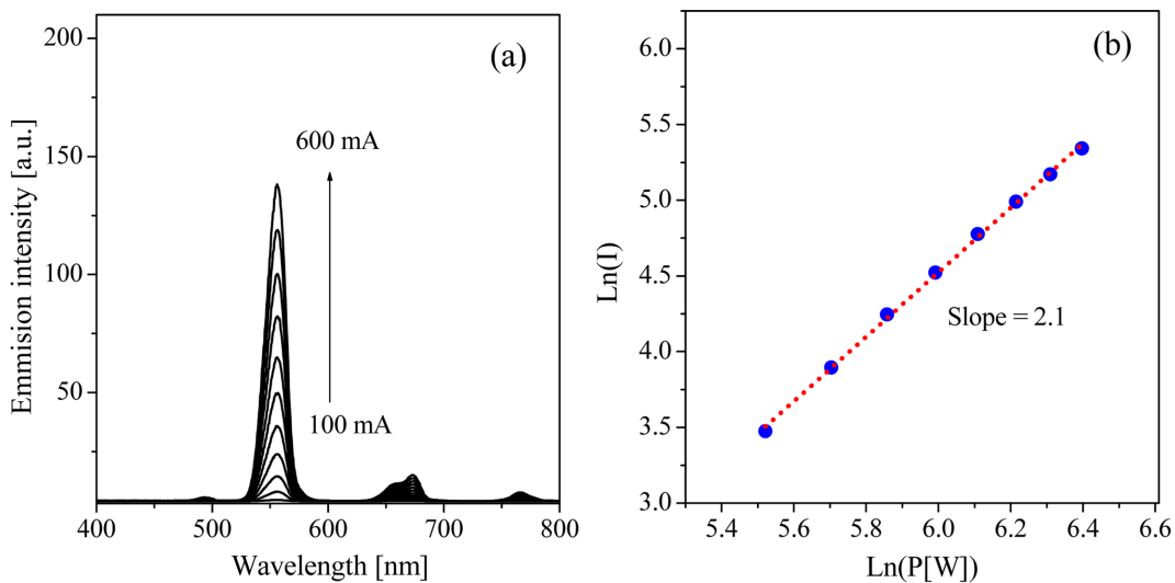
Fig. 6. (a) Emission spectra of SrAl_2O_4:Ho_{0.001}^{3+} phosphors calcined at 1200 °C and (b) Ln-Ln plot of emission intensity as a function of pumping power.
