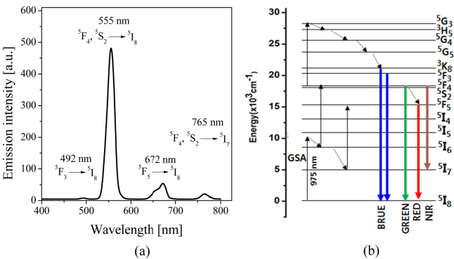
Fig. 1. (a) Emission spectrum of SrAl 2 O 4 :Ho 3+ phosphor under 975 nm excitation and (b) energy level diagram of Ho 3+ activators.
