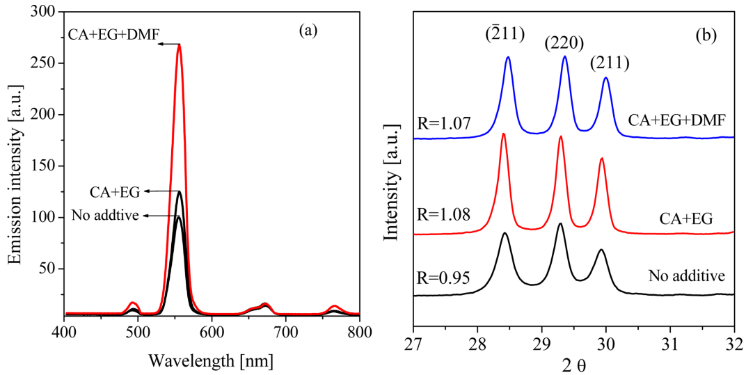
Fig. 7. Effect of organic additives on emission spectra (a) and XRD patterns (b) for SrAl 2 O 4 :Ho 0.001 3+ powders prepared by spray pyrolysis.
