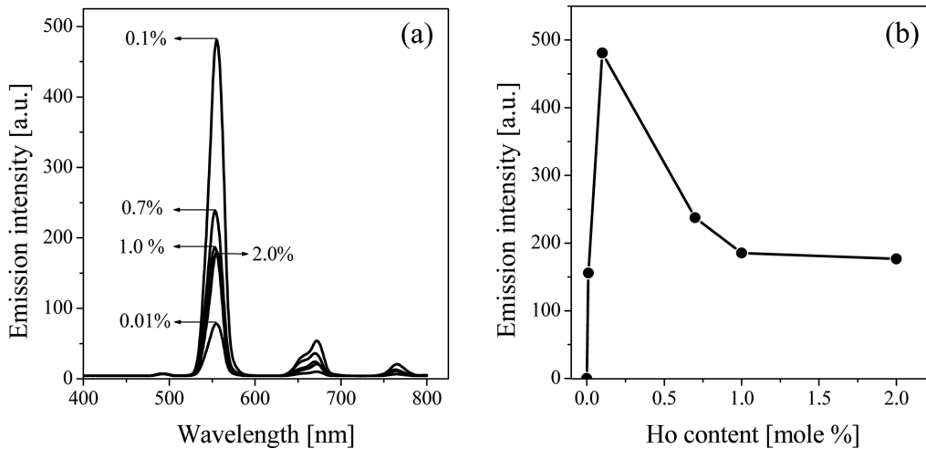
Fig. 4. (a) Emission spectra for SrAl 2 O 4 :Ho 3+ UCs prepared with changing the content of Ho 3+ and (b) changes in the intensity of green emission as a function of Ho 3+ concentration.
