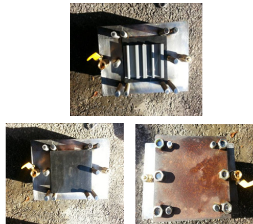
Fig. 9. Test Setup for Profile
