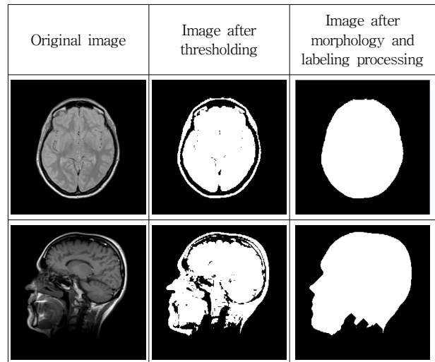
Fig. 3. Images During Object and Background Region Segmentation
