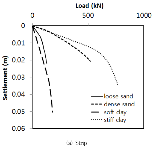
(a) Strip
