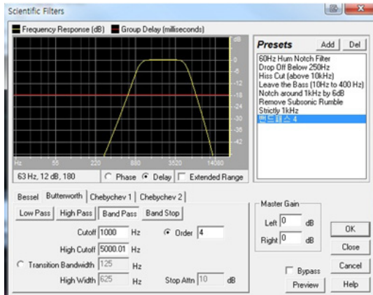
[Fig. 3] BPF implemented through simulation
