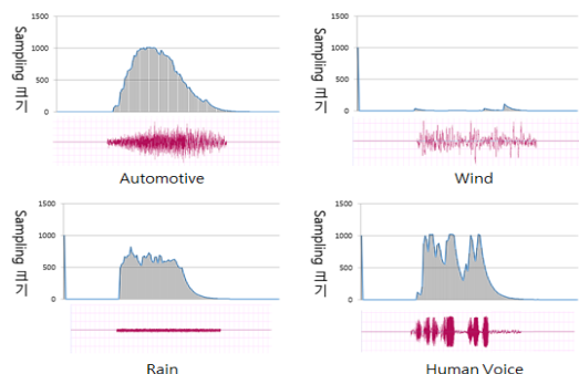
[Fig. 2] sound sampling data
