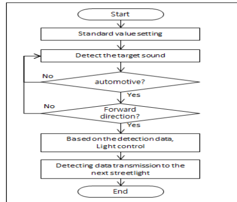
[Fig. 1] system flowchart
