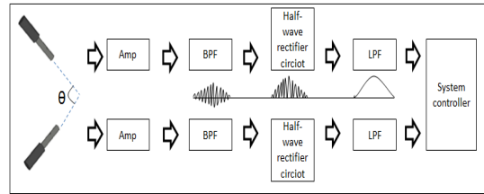
[Fig. 9] automotive sound retrieving system using sensor
