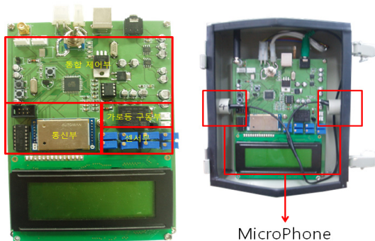
[Fig. 8] System Board
