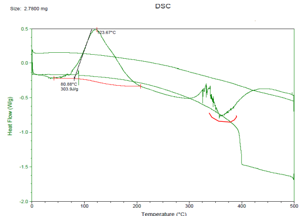
Figure 3. The result of DSC test for hardener mixed liquid epoxy resin.
