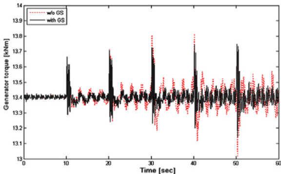
Fig. 12 Comparison of generator torques for pitch PI controller with gain-scheduling
