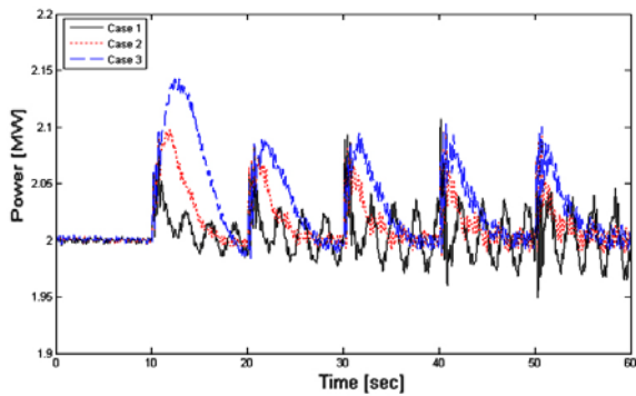
Fig. 5 Comparison of powers for fixed pitch PI controller
