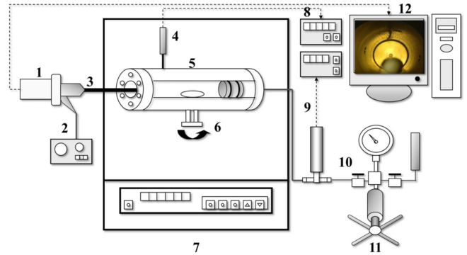
Fig. 1. Schematic diagram of the variable volume view cell (VVVC) apparatus.
