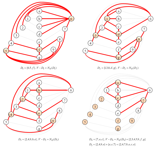
(m) dn(G_{15}) = 3 for G_{15} graph
