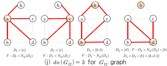
(j) dn(G_{12}) = 3 for G_{12} graph
