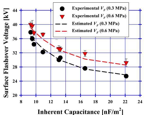
Fig. 6. Comparison of surface flashover voltage on experimental data and empirical formula
