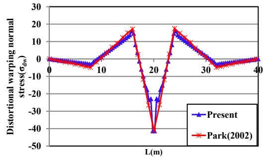
Fig. 4. Distortional warping normal stress along the span length.
