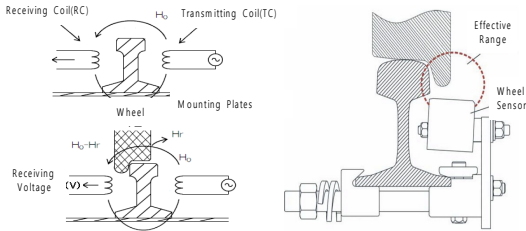
Fig. 1. Magnetic Type Fig. 2. Inductive Sensing Type
