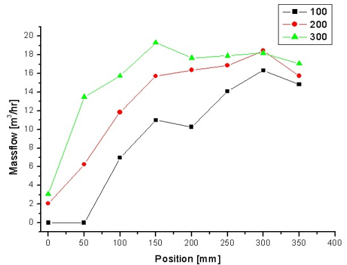
[Fig. 12] Massflow of the Shape of the Ejector Diffuser
