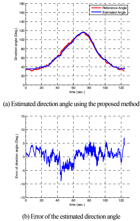
Fig. 8. Experimental result of the direction estimation of underwater acoustic source using the proposed method
