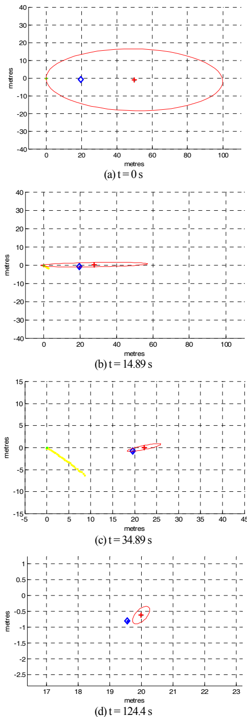
Fig. 9. Experimental result of acoustic source localization
