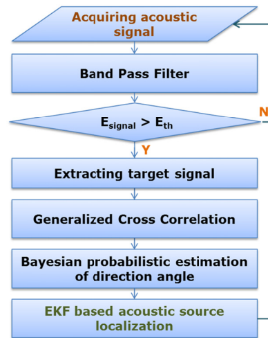
Fig. 2. A flowchart of the proposed acoustic source localization
