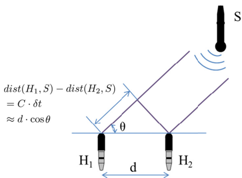
Fig. 1. Time difference of arrivals using two hydrophones
