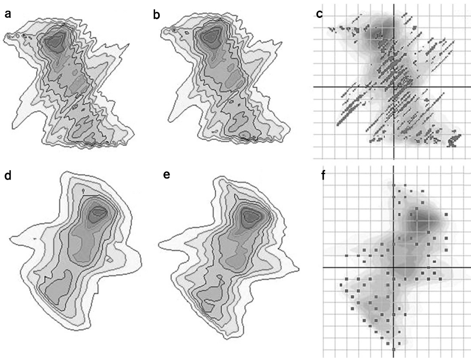
Fig. 1. Gamma analysis of a 6 MV VMAT QA plan at 1%/1 mm using the SNC Patient software. (a) EPID-based measurement, (b) Portal Dose Image Prediction, (c) failed gamma points for EPID-based QA, (d) MapCHECK 2 measurement, (e) calculated dose for MapCHECK 2, and (f) failed gamma points for MapCHECK 2 QA.
