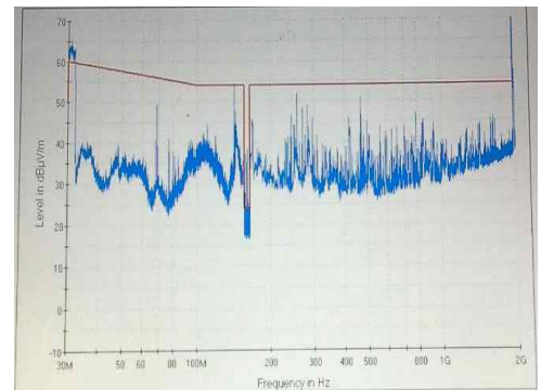
Figure 5: Switchboard Measurement Results on Hanbada (Ultra Log Antenna)
