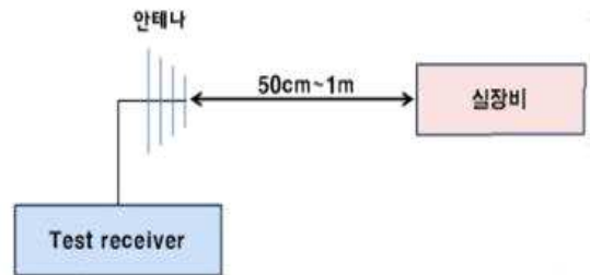
Figure 3: Measurement Method
