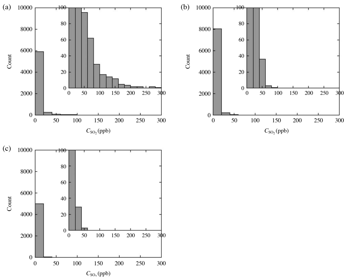
Fig. 3. Histograms of hourly \text{SO}_2 concentrations at the VIF (a), PED (b), and CHO (c) stations (see Fig. 1) from 1 January to 31 December 2011.
