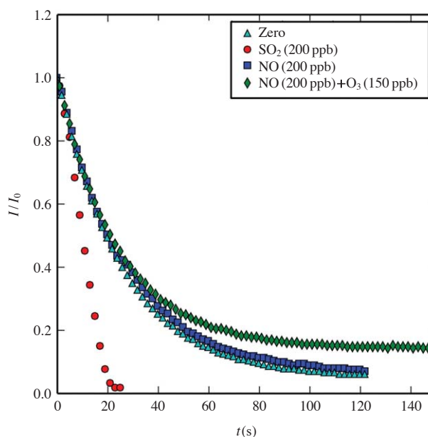
Fig. 2. Response of the ECC ozone sensor when the input gas was changed abruptly from ozone-containing air ( \approx 160 ppb \text{O}_3 ) to various gases indicated in the legend. “Zero” represents air filtered through activated carbon to remove ozone.
