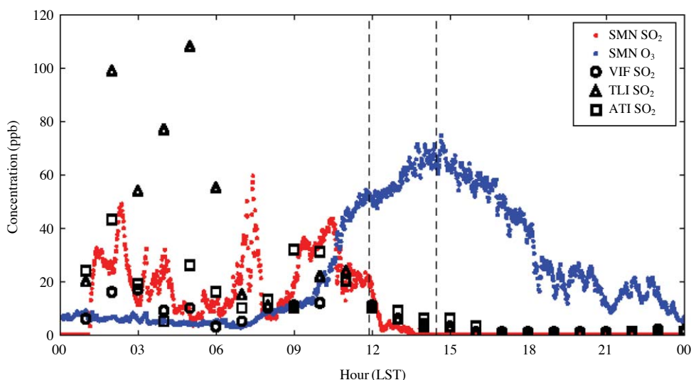
Fig. 7. Trends of O_3 and SO_2 concentrations measured by UV-based equipment at SMN, and SO_2 monitoring data at the VIF, TLI, and ATI air-monitoring stations in the northern part of MCMA on 14 March 2012.
