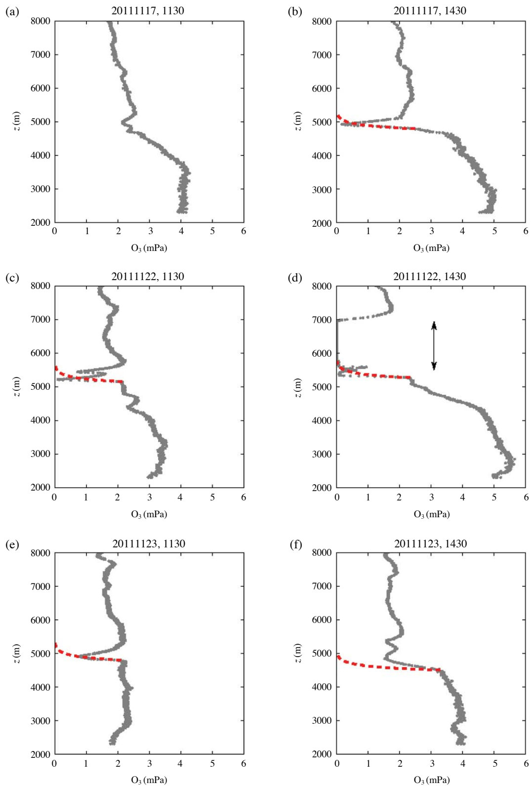
Fig. 4. Vertical profiles of the partial pressure of O_3 during the campaign in November 2011. The nominal launch times are LST. The height z is ASL. The dashed lines indicate expected responses of the ECC ozone sensor if the O_3 concentration dropped abruptly to zero at the height corresponding to the bottom of the curves.
