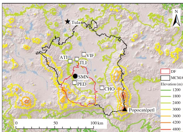
Fig. 1. Map of the Mexico City Metropolitan Area (MCMA). The region denoted by DF is the Federal District. The black circle is the SMN balloon launching site, and the white squares are stations of the Mexico City air-monitoring network (RAMA): VIF, Villa de las Flores; PED, Pedregal; CHO, Chalco; TLI, Tultitlan; ATI, Atizapan.
