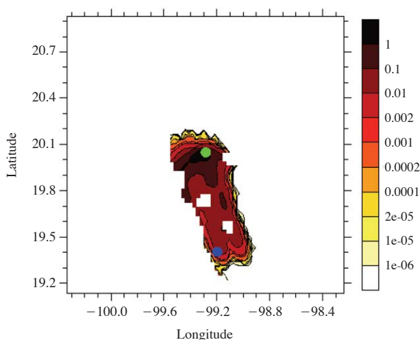
Fig. 8. Result of WRF+FLEXPART numerical simulation for 12:00 LST (18:00 UTC) on 14 March 2012. One million particles totalling a unit mass were released from the Tula industrial complex (green circle) for 20 h beginning at 01:00 UTC on 14 March 2012. The release height was between 100 and 1000 m AGL. The contours represent the concentration in the horizontal section at 2500 m ASL. The white defect cells indicate terrain above 2500 m ASL. The coordinate values (in degrees) are longitude (positive in the east) and latitude (positive in the north). The blue circle indicates the location of SMN.
