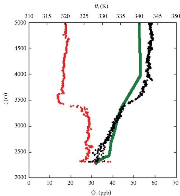
Fig. 6. Vertical distribution of O 3 concentration and equivalent potential temperature for the 11:30 LST launch on 14 March 2012. Black dots, O 3 concentration; red dots, equivalent potential temperature; green curve, influence of the SO 2 plume on O 3 concentration (average of 11:00 and 12:00 LST results simulated by WRF-FLEXPART).
