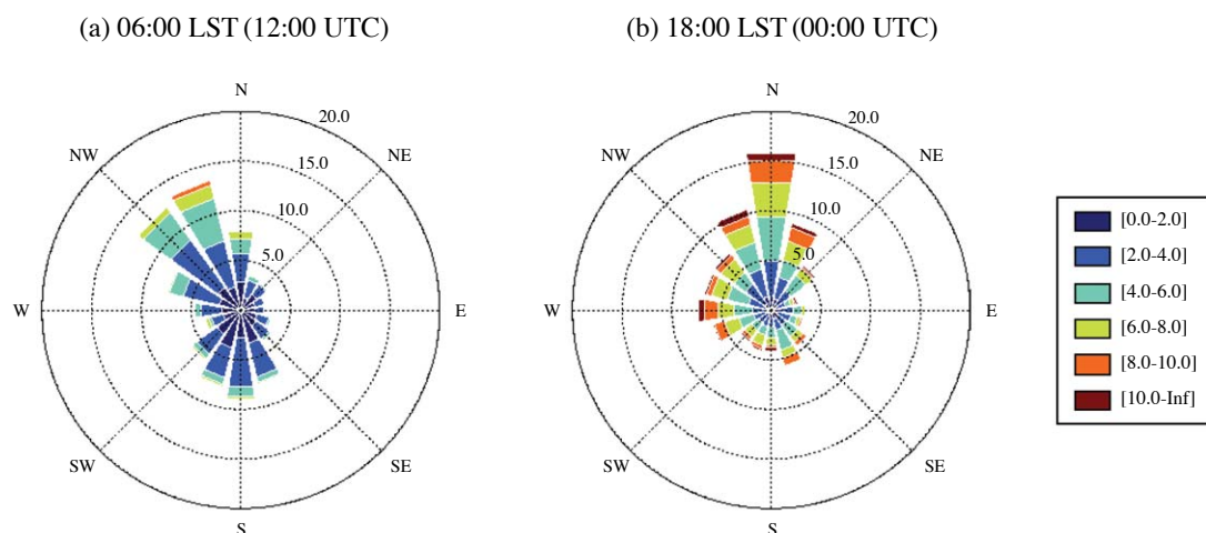
Fig. 10. Wind rose obtained by averaging sounding data at elevations ranging from 2343 to 2463 m ASL (30-150 m AGL at SMN). The unit for wind speed is metres per second and wind-direction frequency is expressed in percent. The data source is routine sounding data collected at SMN from 2006 to 2010.
