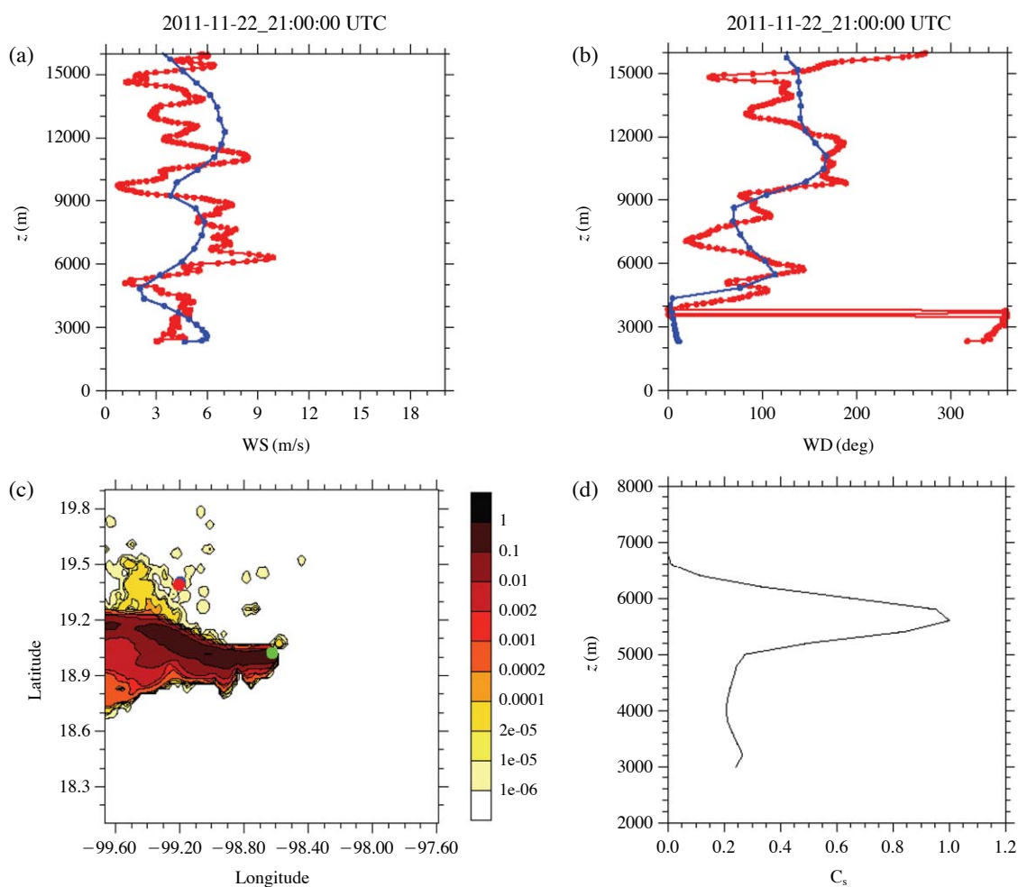
Fig. 5. Results of WRF+FLEXPART numerical simulation for 15:00 LST (21:00 UTC) on 22 November 2011. The height z is ASL. (a, b) Vertical profiles of wind speed and wind direction (blue, WRF; red, observation). (c) Forward particle release simulation by FLEXPART. One million particles totalling a unit mass were released from the summit of Popocatepetl for 20 h beginning at 19:00 LST on 21 November 2011. The release height was between 5426 m ASL (summit) and 5926 m ASL. The contours represent the concentration ( \text{m}^{-3} ) in the horizontal section at 5500 m ASL. The coordinate values (in degrees) are longitude (positive in the east) and latitude (positive in the north). The red and green circles indicate the locations of SMN and the Popocatepetl summit, respectively. (d) Vertical profile of the number of particles concentrically located 60 to 80 km from the centre of Popocatepetl. The particle number C_s is normalized by the maximum value at 5500 m ASL.
