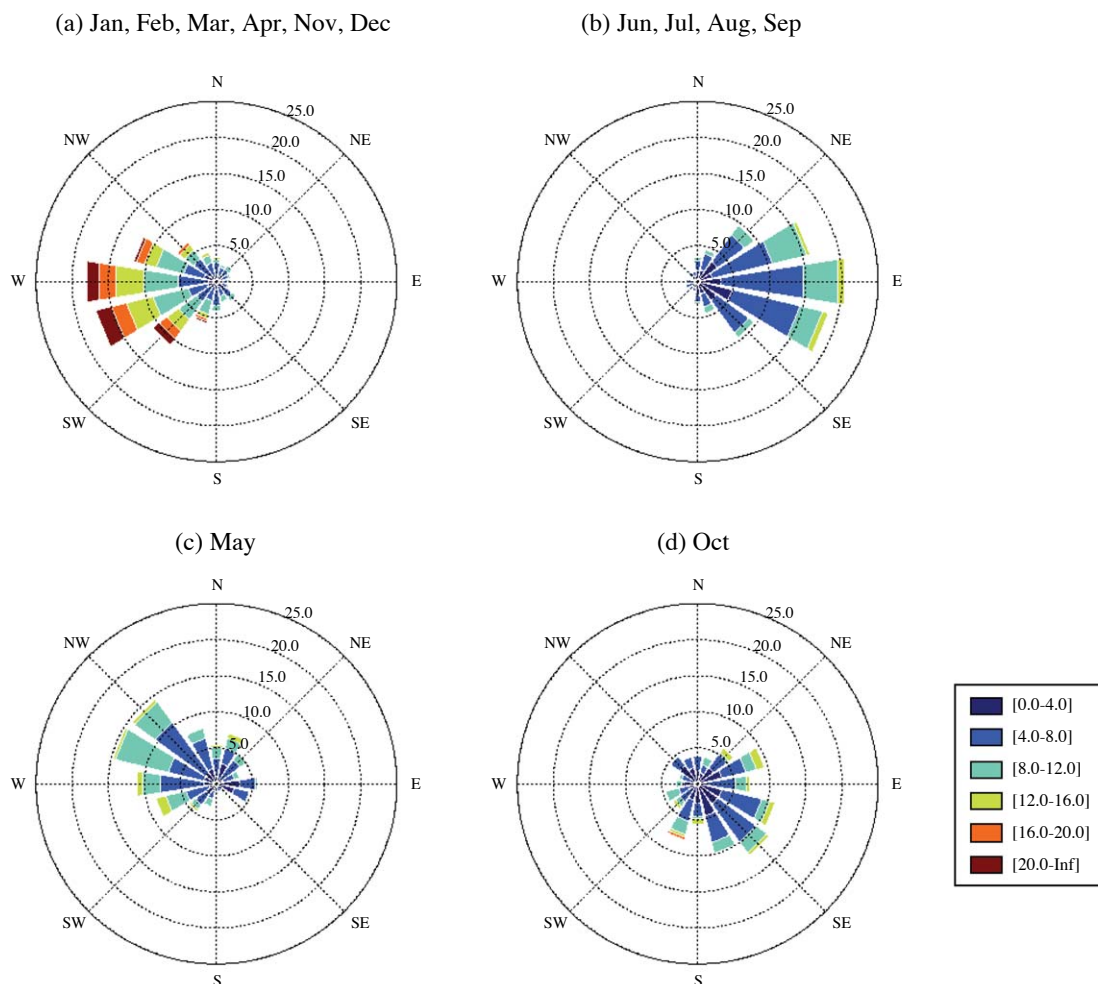
Fig. 9. Wind rose obtained by averaging sounding data at elevations ranging from the Popocatepetl summit to 1000 m above the summit. The unit for wind speed is metres per second and wind-direction frequency is expressed in percent. The data source is routine sounding data collected at SMN from 2006 to 2010. Months with similar distribution are grouped together.
