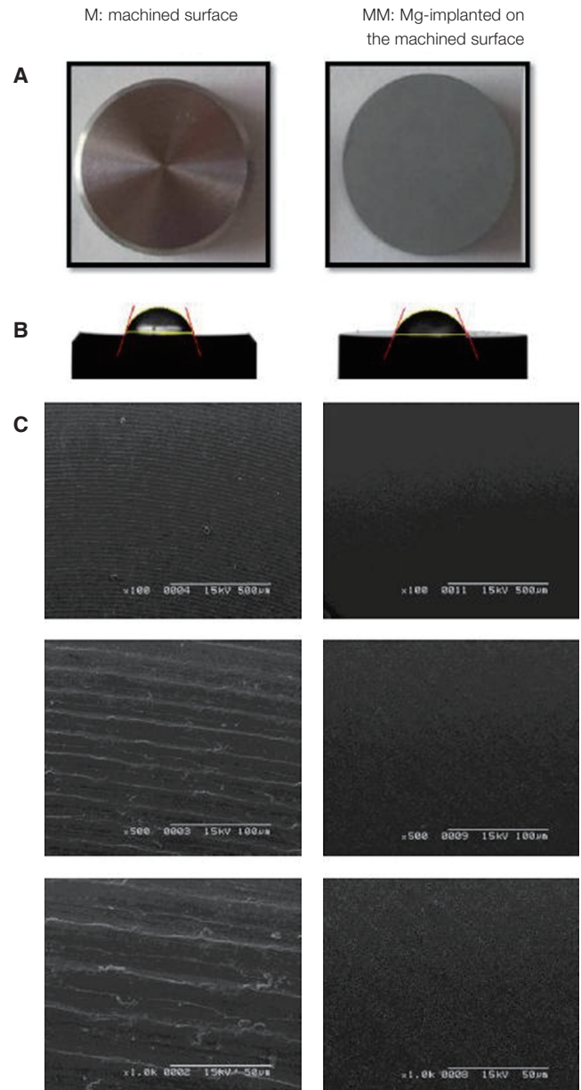
Fig. 1. Titanium disc specimens (Shinheung, Co, Korea) of 10 mm diameter x 3 mm thickness (A). Machined surface (M) is more hydrophobic than the Mg-implanted on the machined surface (MM) contact angles are shown in Table 3 (B). SEM images of the different titanium surfaces are shown (C)(x100, x500 and x1,000).
