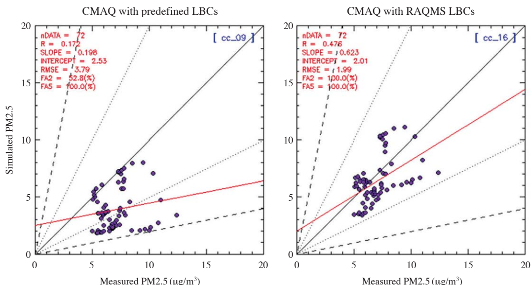
Fig. 5. Scatter diagram of regional average PM 2.5 concentration for western region for August 30-September 1, 2006. CMAQ with predefined (left) and RAQMS (right) LBCs are compared with the EPA AQS PM 2.5 data.
