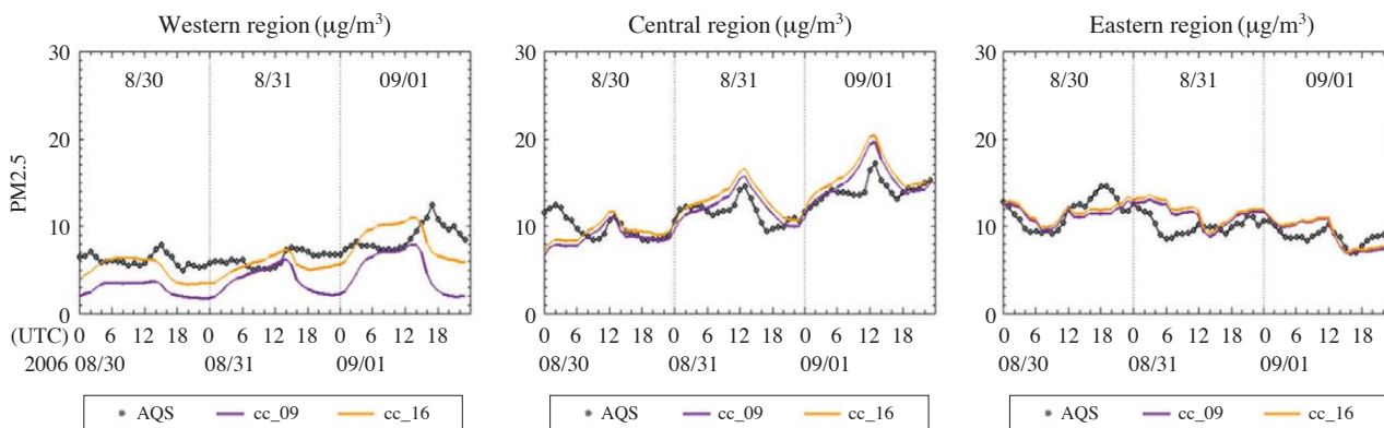
Fig. 4. Time series of CMAQ regional average PM 2.5 concentration for three regions (western: left, central: middle, eastern USA: right), compared to AQS hourly PM 2.5 measurements. Purple and orange lines are the PM 2.5 concentration from CMAQ with predefined and RAQMS LBCs, respectively. Black circle lines are the observed PM 2.5 .
