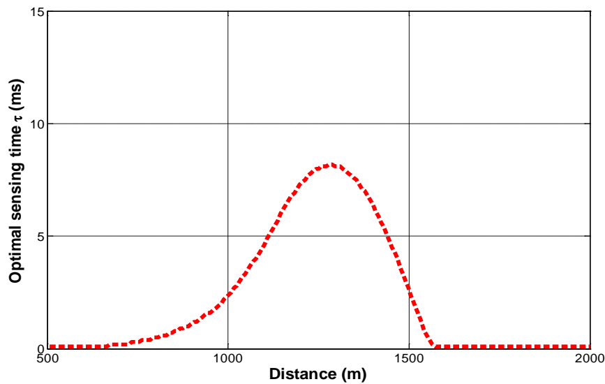
Fig. 3. Optimal sensing time that maximize the achievable throughput
