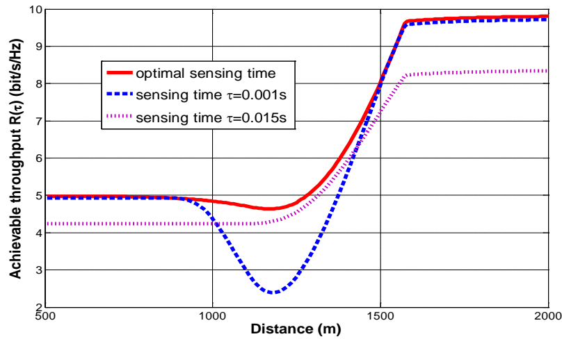
Fig. 4. The achievable throughput of different sensing time
