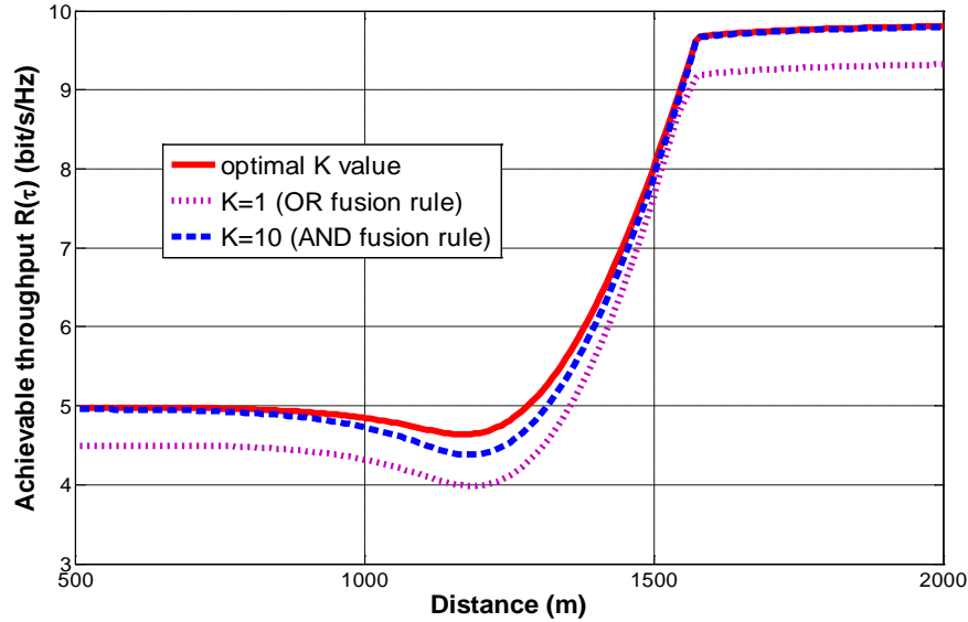
Fig. 5. The achievable throughput of different K values
