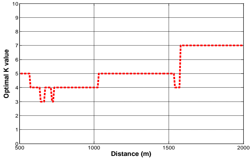
Fig. 2. Optimal K that maximize the achievable throughput
