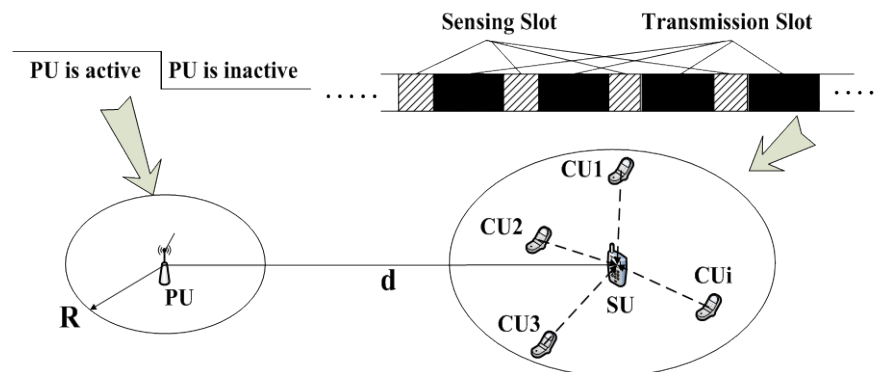
Fig. 1. System model of cognitive radio network (R: radius of PU; d: the distance between PU and SU)
