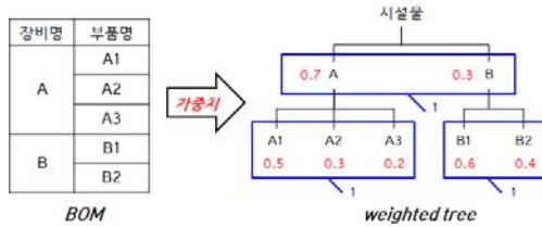
Figure 1: Example for BOM and weighted tree
