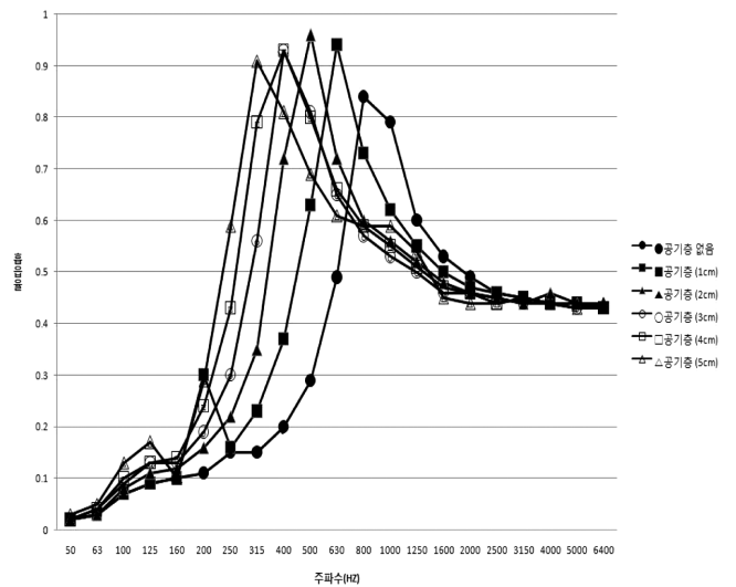
Fig. 9. Effect of the air cavity depth on the absorption coefficients of composite of silica aerogel and pulps.
