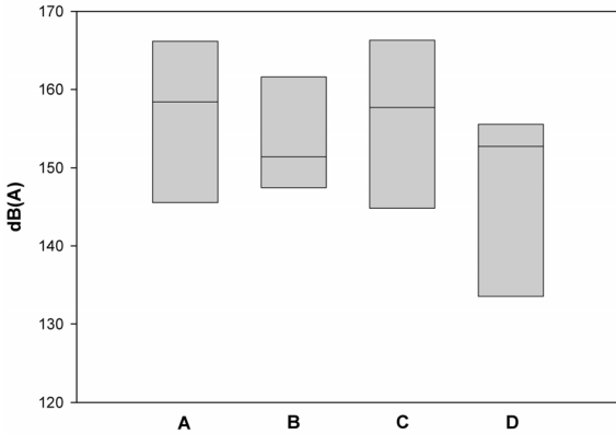
Figure 2. Comparison of peak noise level by sampling point on the tanks(A: Loading soldier(n=6), B: Shooter(n=8), C: Upper side of tank(n=6), D: Waiting soldier(n=8))
