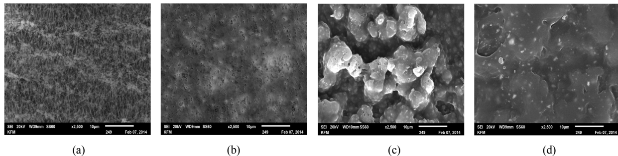
Figure 2. SEM photographs of selectively permeable membranes: (a) Single e-PTFE, (b) Treated e-PTFE, (c) Bi-component e-PTFE, (d) PET.
