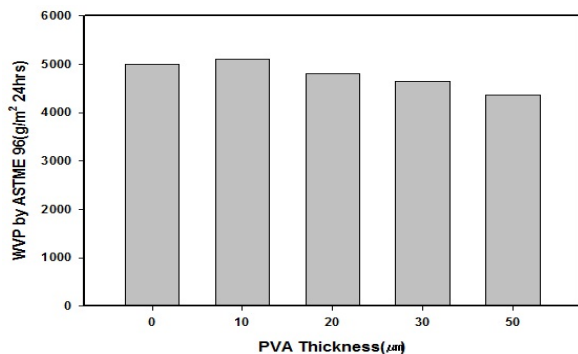
Figure 3. Breathability of selectively permeable membranes with various PVA coating thickness.
