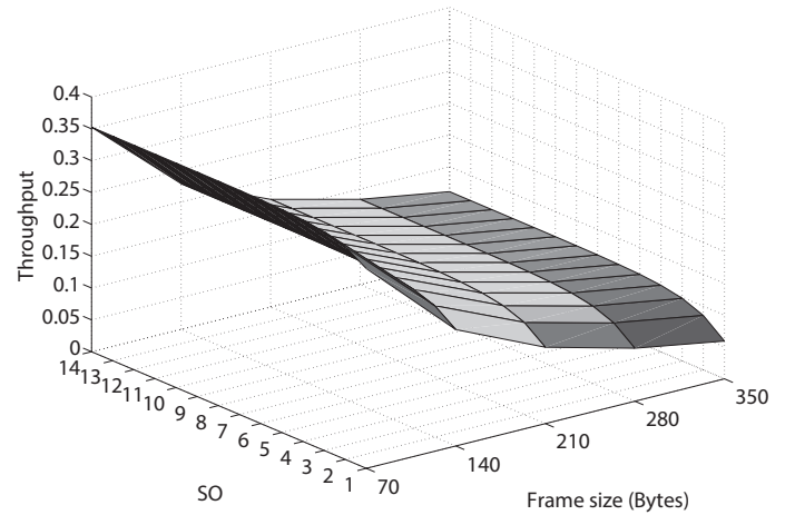
Fig. 3: Throughput variation as a function of superframe and data frame sizes.
