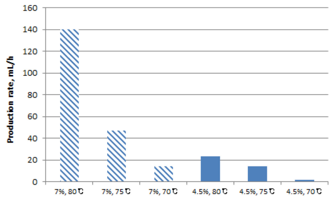
Fig. 4. The amount of fresh water according to changes in temperature and concentration using saturated vapor pressure.
