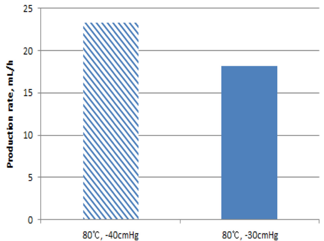
Fig. 5. The amount of fresh water as pressure changes.
