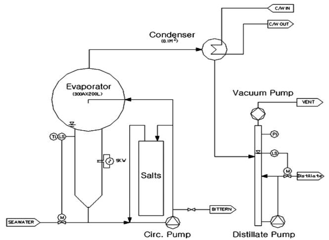
Fig. 1. Plan of reduced pressure evaporation.
