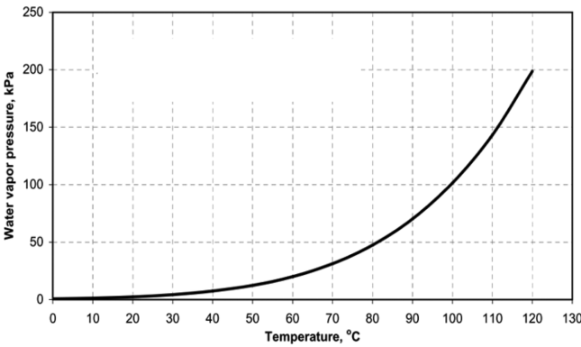
Fig. 3. Saturated vapor pressure in accordance with temperature change.
