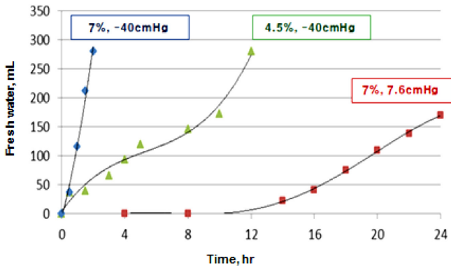
Fig. 7. Time and fresh water acquired for example (at 80 °C).
