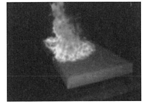
[RS1 at the beginning and at 4min 30s] - Max HRR of 447.93 kW - Max SPR of 9.81 m 2 /s
