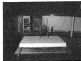
[RS1 at the beginning and at 4min 30s] - Max HRR of 447.93 kW - Max SPR of 9.81 m 2 /s
