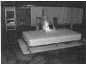
[AS1 at the beginning and at 4min 30s] - Flashover occur - Max SPR of 41.56 m 2 /s
