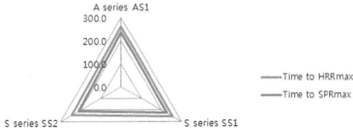
Figure 4. Correlation on HRR & SPR of Specimen with Flashover
