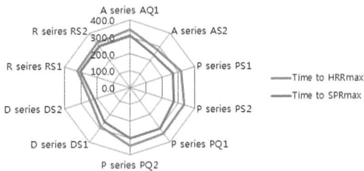
Figure 5 Correlation on HRR & SPR of Specimen without Flashover
