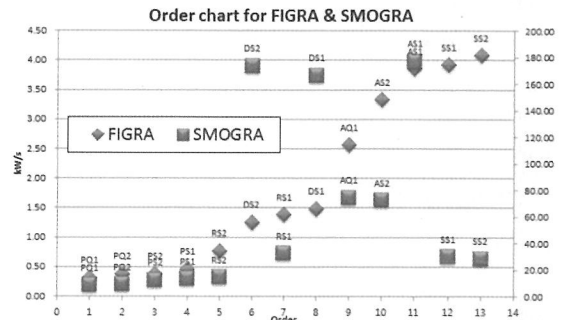
Figure 3. Test Result as FIGRA order
