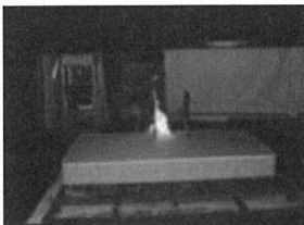
[PS1 at the beginning and at 4min 30s] - Max HRR of 146.16 kW - Max SPR of 3.42 m 2 /s
