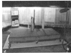
[DS1 at the beginning and at 4min 30s] - Max HRR of 429.49 kW - Max SPR of 42.03 m 2 /s
