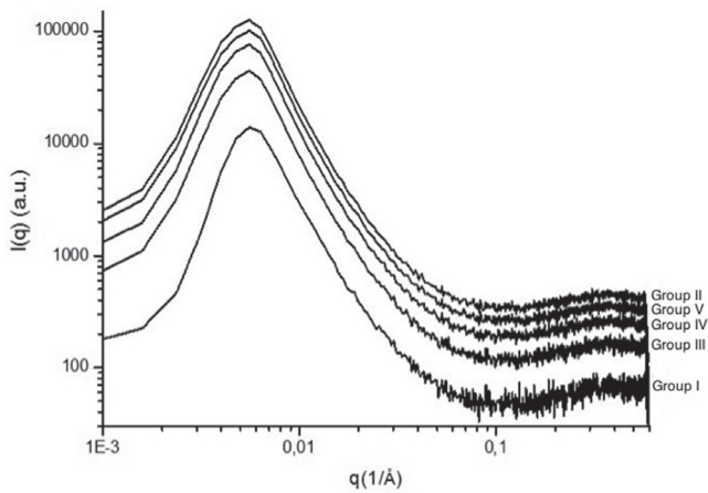
Fig. 1. SAXS patterns of the groups that were analyzed; q , magnitude of the scattering vector.
