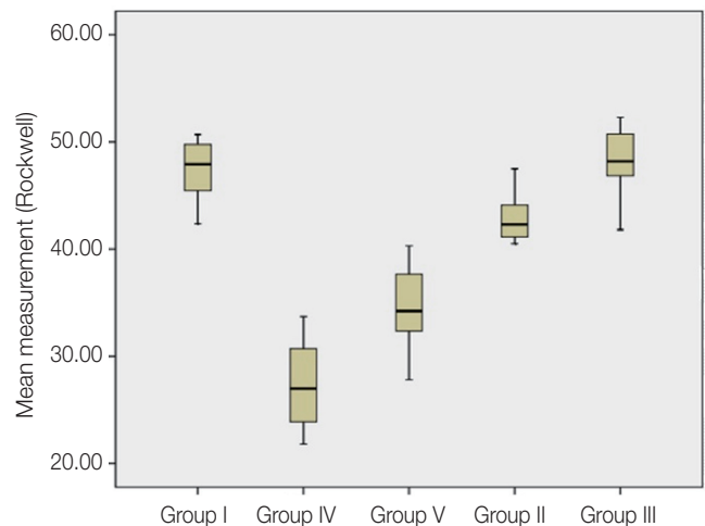
Fig. 3. Statistical results of the Rockwell measurements of the groups. Maximum hardness was measured in Group III (non-annealed) and minimum value was seen in Group IV (argon-annealed).
