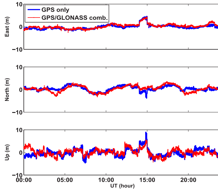
Fig. 3. Comparison of the positioning results at the GRAS reference station.
