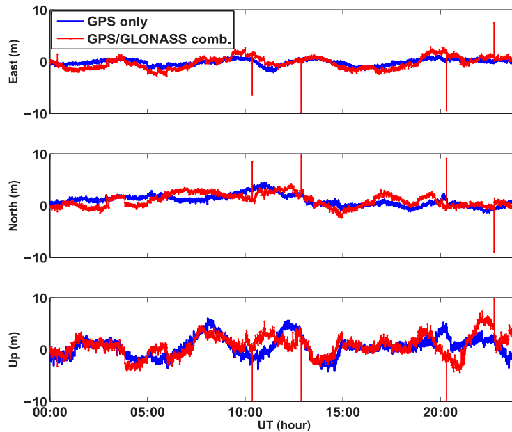
Fig. 5. Comparison of the positioning results at the KOHG reference station.
