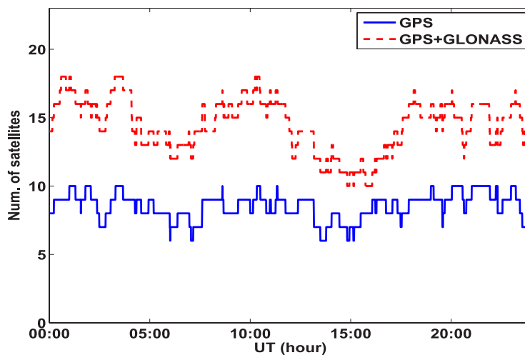
Fig. 2. Comparison of the number of GPS satellites and the number of combined GPS/GLONASS satellites, observed at the GRAS reference station.
