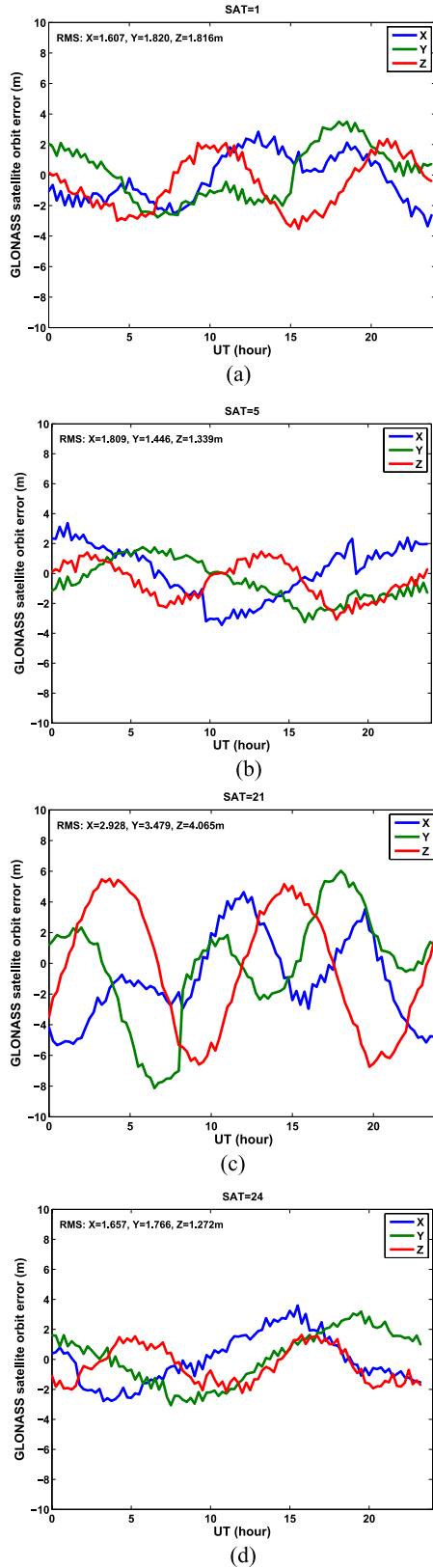
Fig. 1. Orbit error between the GLONASS satellite orbits calculated using broadcast ephemeris and the precise ephemeris: (a) GLONASS satellite 1, (b) GLONASS satellite 5, (c) GLONASS satellite 21, and (d) GLONASS satellite 24.
