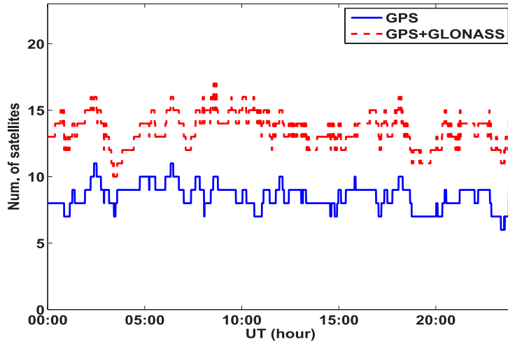
Fig. 4. Comparison of the number of GPS satellites and the number of combined GPS/GLONASS satellites, observed at the KOHG reference station.
