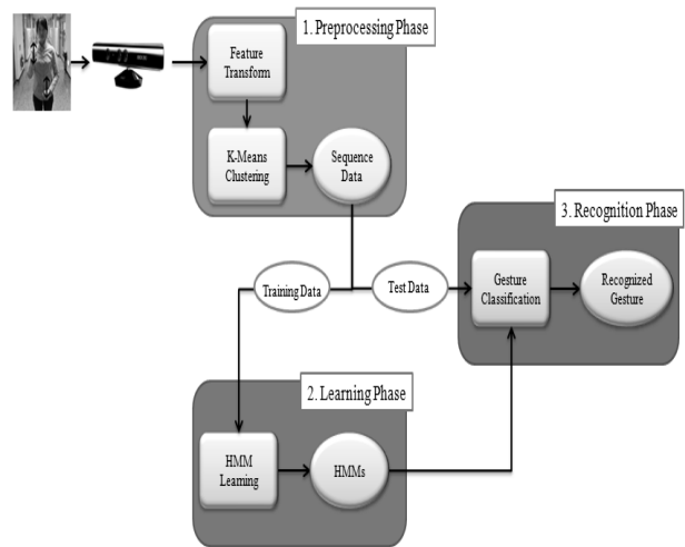
Fig. 1. Overall process of arm gesture recognition
