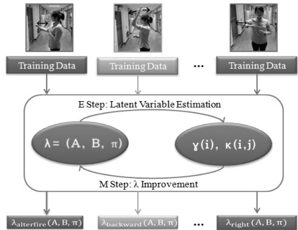
Fig. 5. Baum-Welch algorithm for learning HMMs
