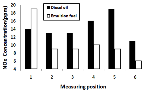
Figure 14: NOx comparisons between diesel and the emulsion of water mixing percent of 16.7% and fuel consumption reduction of 12%
