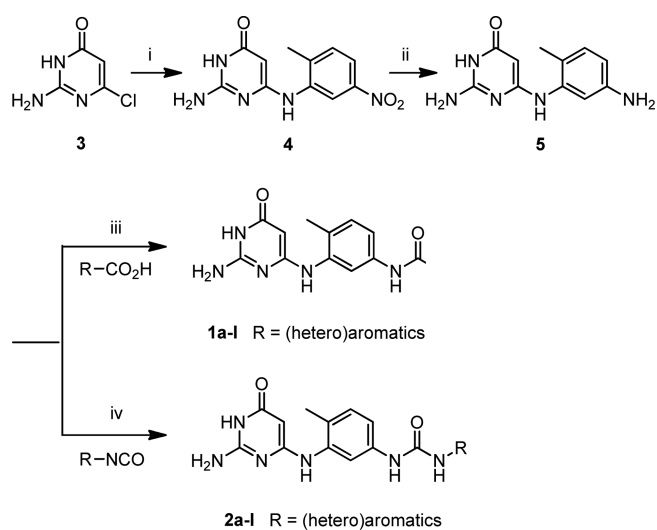
Scheme 1. Reagents and reaction conditions: (i) 2-methyl-5-nitroaniline, 170 °C, 3 h; (ii) 5% Pd/C, \text{H}_2 , MeOH, rt, 2 h; (iii) HOBt, EDCl, \text{Et}_3\text{N} , DMF, 90 °C, 12 h; (iv) THF, rt, 4 h.
