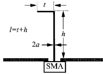
Fig 3. Configuration of inverted F antenna.
