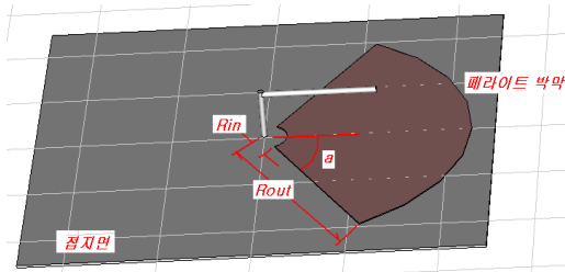
Fig. 4. The configuration of a inverted L antenna on the ground plane with ferrite thin film.
