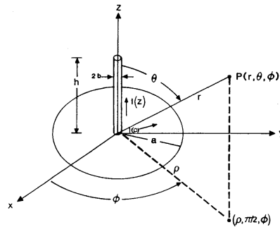
Fig. 1. Configuration of a basic monopole antenna.
