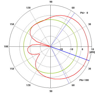
Fig. 5. Radiation pattern of the 'Case B-4' antenna.
