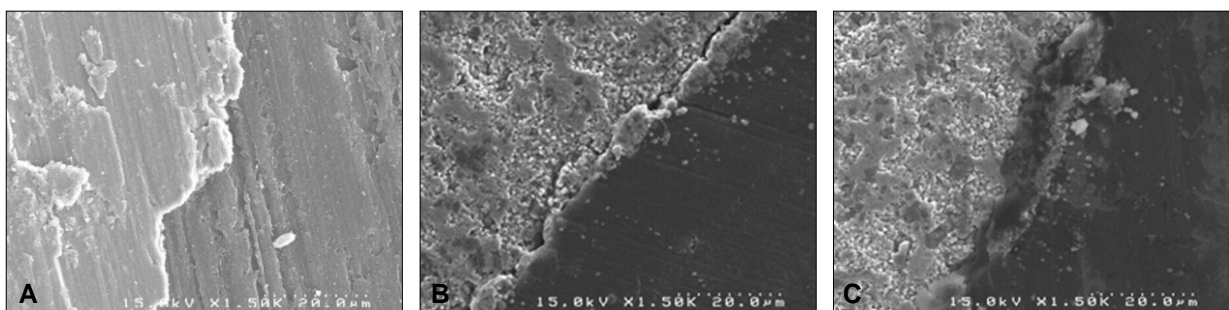
Fig. 6. Scanning electron micrographs of bone to implant contact taken 4 weeks after insertion. A: Group T, An unmineralized zone separated the mineralized bone from the implant surface (×1,500). B: Group Z, Interface tissue between calcified bone and implant (×1,500). C: Group ZS, A dense amorphous layer was located at the implant surface (×1,500).
