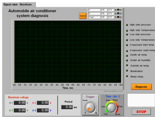
[Fig. 13] Refrigerant and Connection Condition Change Graph Construction and Diagnosis Program
